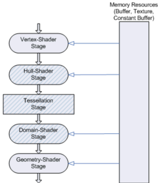
Figure 12: Hardware Tessellation pipeline from Direct3D 11 [25]
